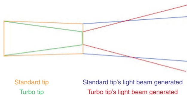
FIGURE 1. Geometric behavior of light tips. When the tip's exit diameter is smaller than the entry diameter, a narrower light beam is created. In the near portion of the light beam, the intensity is greater than that emitted by a standard tip. However, at a distance of 4–5 mm, the light intensity decreases and is actually less than that emitted by a standard tip.
